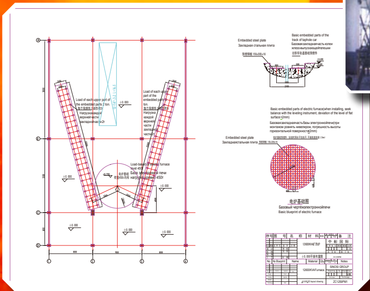
▲ 熔炼炉平面图 Smelting furnace layout
